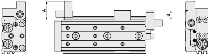
Rubber Stopper (AS, AT, A) (mm)
