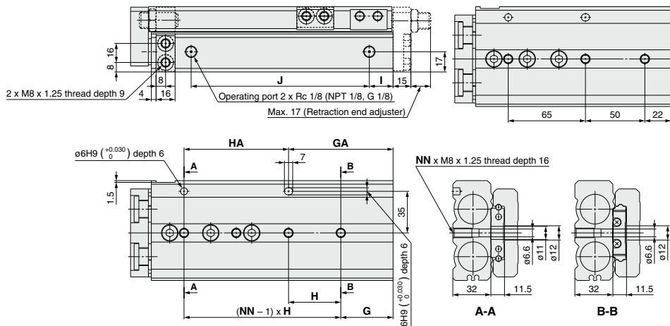
Bottom view of MXQ25L-75
