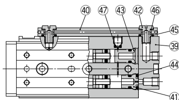
Axial piping type
