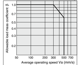
Graph (1) Allowable Load Mass Coefficient: β
