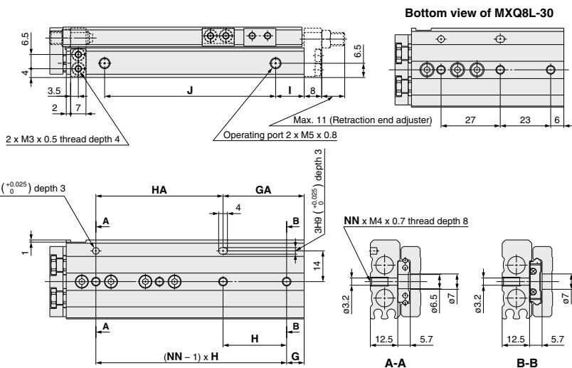
Bottom view of MXQ8L-30
