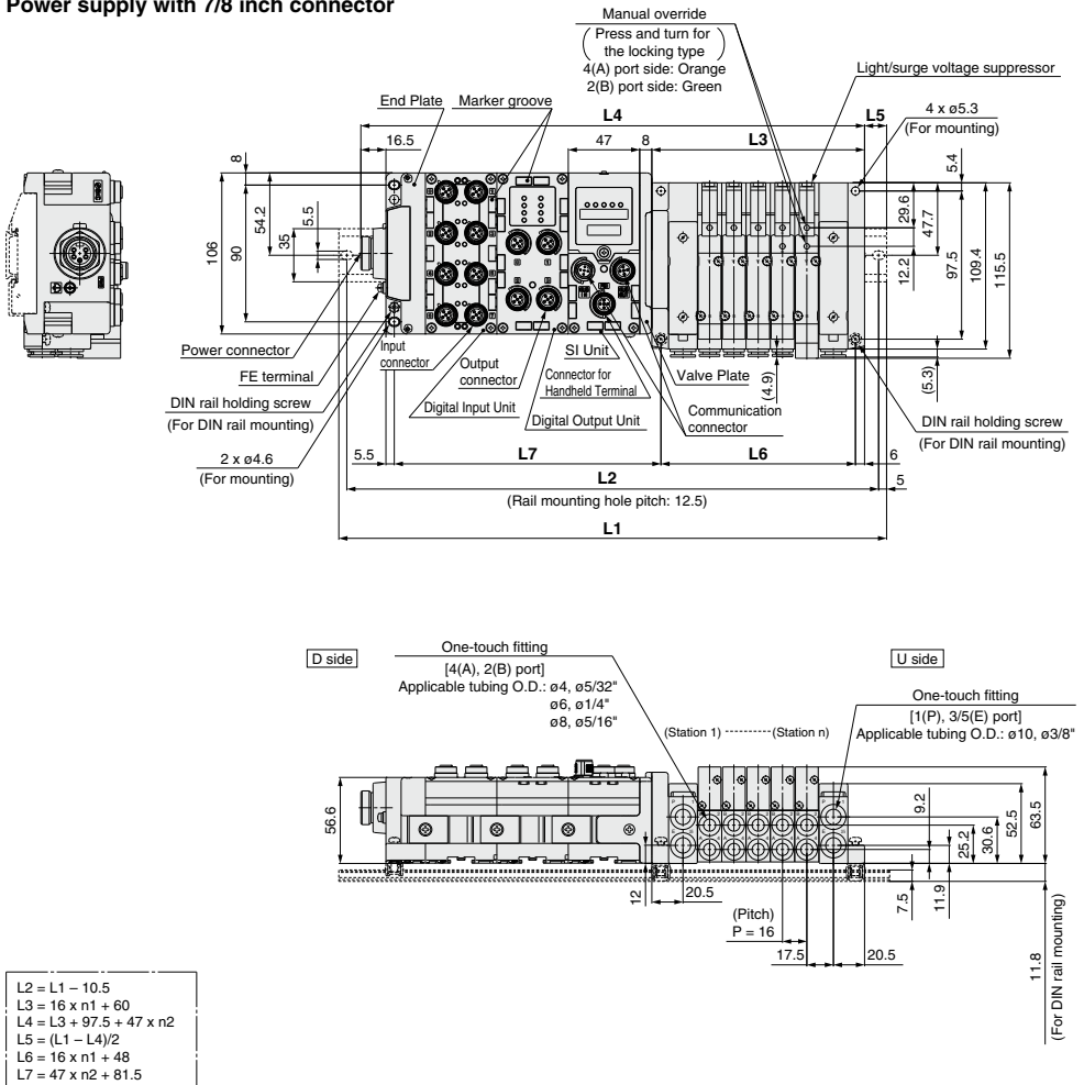
L1: DIN Rail Overall Length
