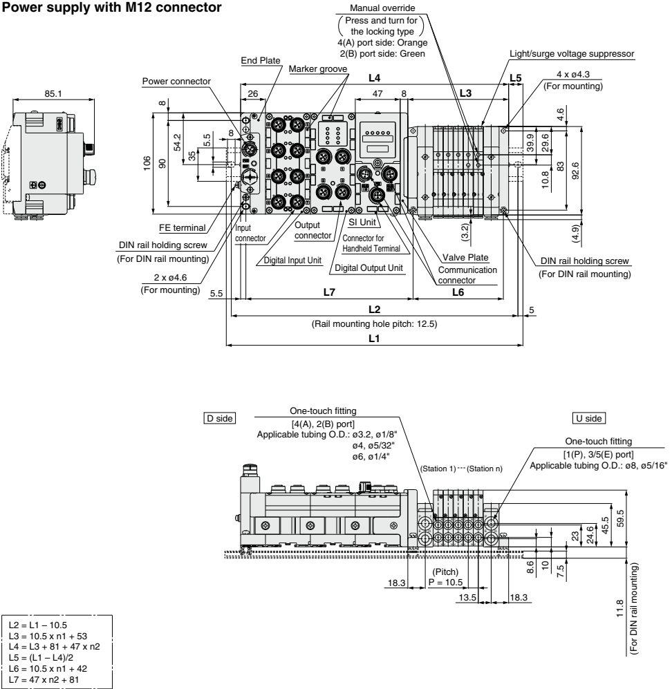
L1: DIN Rail Overall Length
